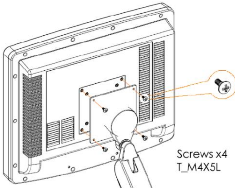
Figure 31 ARCHMI-9XXB VESA MOUNTING
