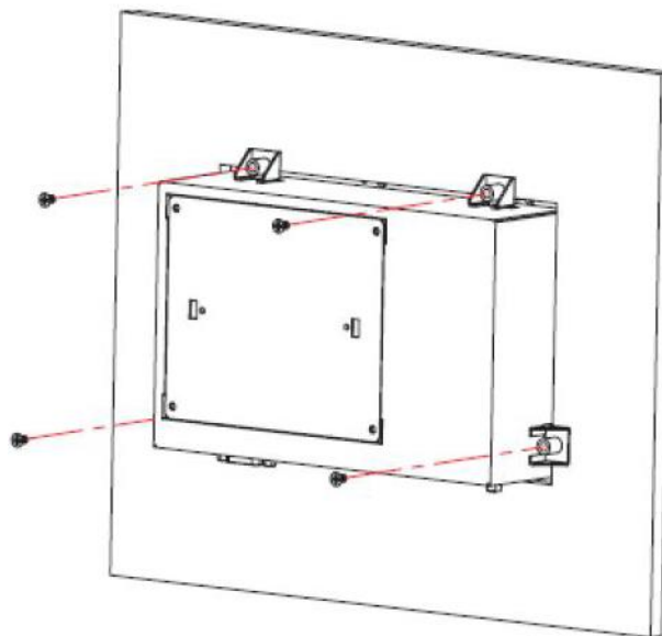
Figure 32 ARCHMI-9XXB PANEL MOUNTING
