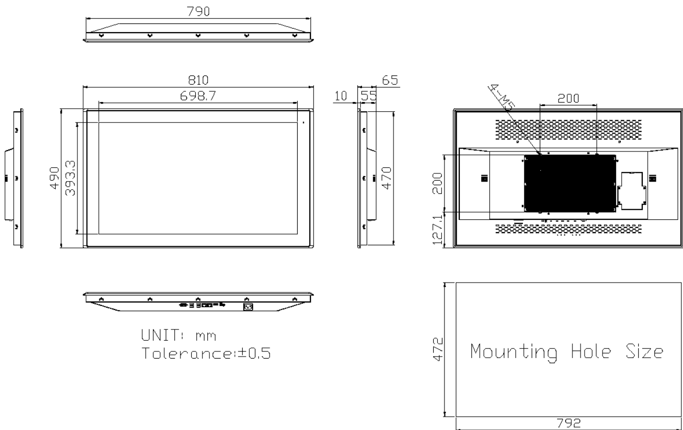
Figure 10 Dimensions of ARCHMI-932BP
