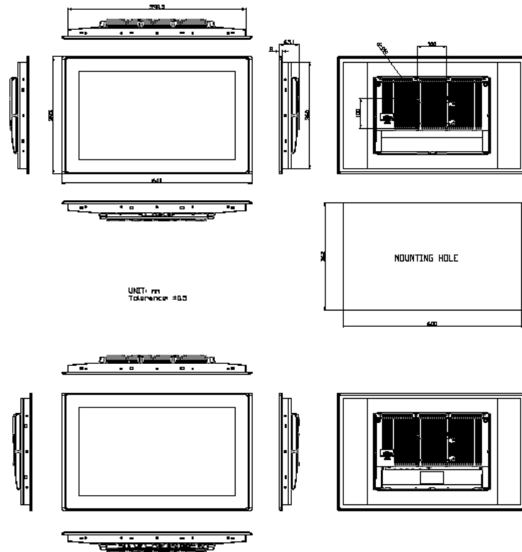
Figure 9 Dimensions of ARCHMI-924BP
